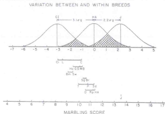
Figure 2—Breed cross means ( F_1 crosses, lower axis) and genetic variation between and within breeds ( \sigma g , standard deviation in breeding value, upper axis) for marbling score. See Table 1 for abbreviations.
